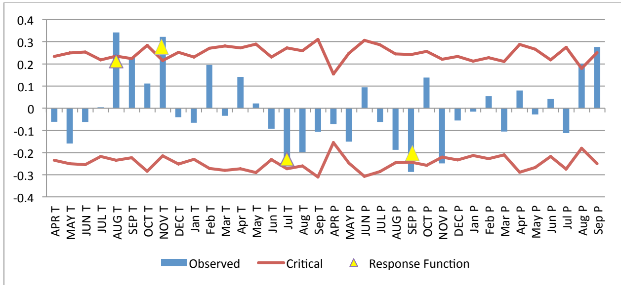
Fig. 2 Results of the climate analysis comparing annual tree-ring growth to historical temperature (T) and precipitation (P) variables from the Saskatoon climate station. Bars represent the degree of correlation between growth and the climate variable, with anything surpassing the linear thresholds being considered significantly correlated. The uppercase letters (i.e. APR T) present variables from the previous year (for example, the conditions of the previous fall often have an impact on tree growth during the current year).
