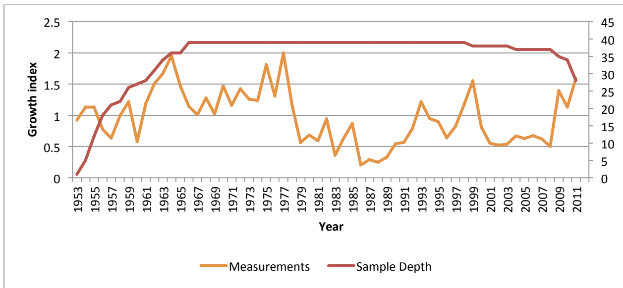
Fig. 1 Master chronology for white spruce (12AFL200) at the Sprayed Spruce site. A standardized measurement of one indicates an average year of growth (in this case, 1.96 mm) while any value above or below one indicates a year of above or below average growth. Sample depth (right axis) is the number of samples averaged to produce the ring measurement for that year.
