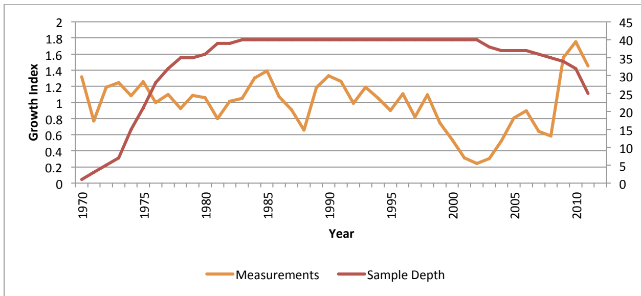
Fig. 1 Master chronology for white spruce (12AHL200) at the (C)overt site. A standardized measurement of one indicates an average year of growth (in this case, 3.36 mm), while any value above or below one indicates a year of above or below average growth. Sample depth is the number of samples averaged to produce the ring measurement for that year.
