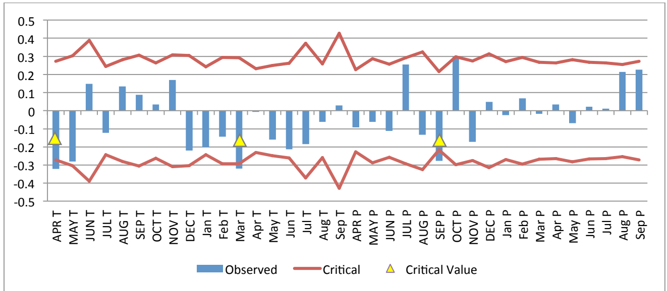
Fig. 2 Results of the climate analysis comparing annual tree-ring growth to historical temperature (T) and precipitation (P) variables from the Saskatoon climate station. Bars represent the degree of correlation between growth and the climate variable, with anything surpassing the linear thresholds being considered significantly correlated. The uppercase letters (i.e. APR T) present variables from the previous year (for example, the conditions of the previous fall often have an impact on tree growth during the current year).
