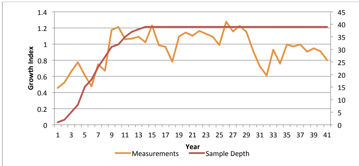
Fig. 1 Master chronology for white spruce (12AIL200) at the Strelieff farm. A standardized measurement of one indicates an average year of growth, while any value above or below one indicates a year of above or below average growth. Sample depth is the number of samples averaged to produce the ring measurement for that year.
