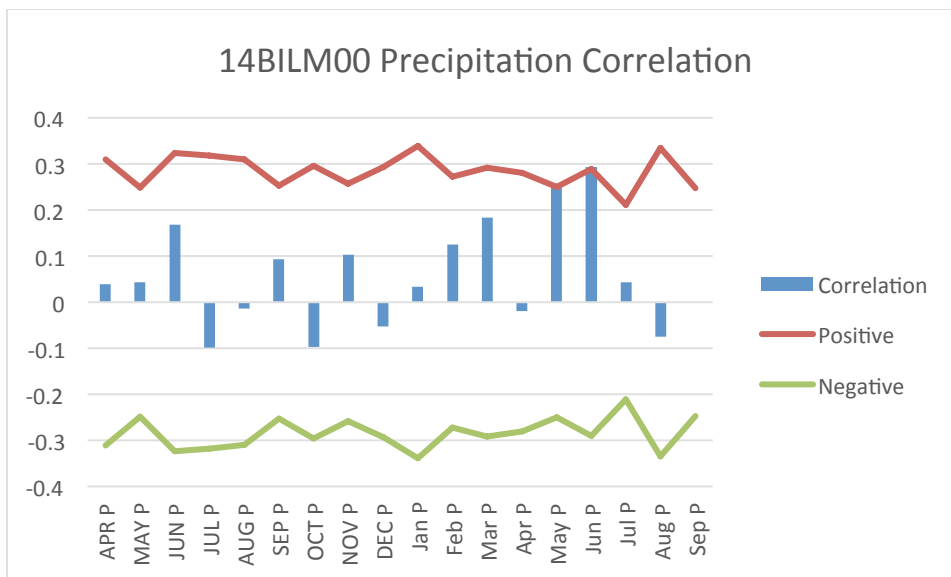
Figure 3: Results of the climate analysis comparing annual tree-ring growth to historical precipitation variables from Waseca, SK.
