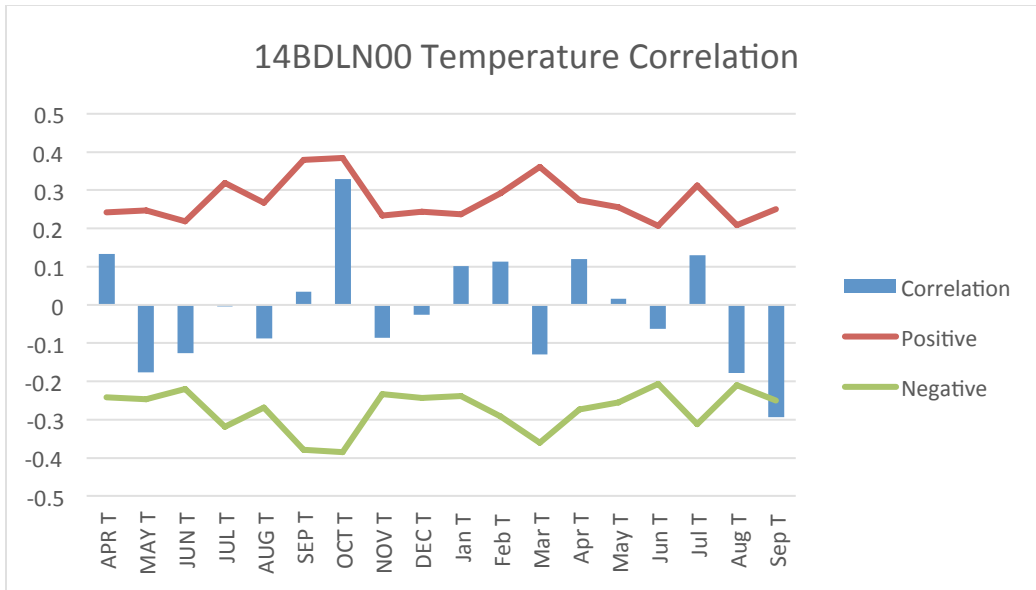
Figure 2: Results of the climate analysis comparing annual tree-ring growth to historical temperature variables from Saskatoon, SK. The bars represent the degrees of correlation between the tree growth and the climate variable. The places where the bars cross the linear threshold are considered significantly correlated. The uppercase letters (ie., APR) label the previous years' variables.
