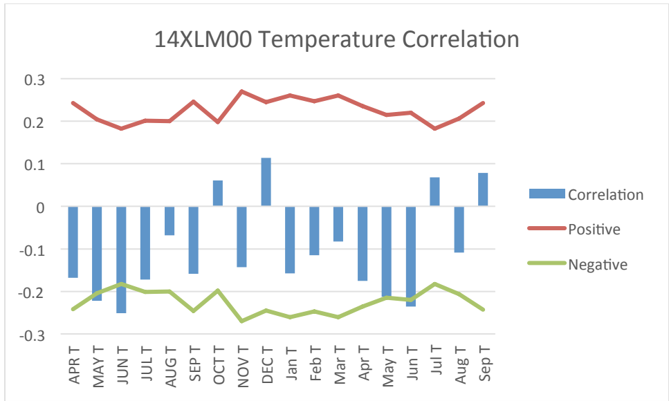
Figure 2: Results of the climate analysis comparing annual tree-ring growth to historical temperature variables from Outlook, SK. The bars represent the degrees of correlation between the tree growth and the climate variable. The places where the bars cross the linear threshold are considered significantly correlated. The uppercase letters (ie. APR) label the previous years' variables.
